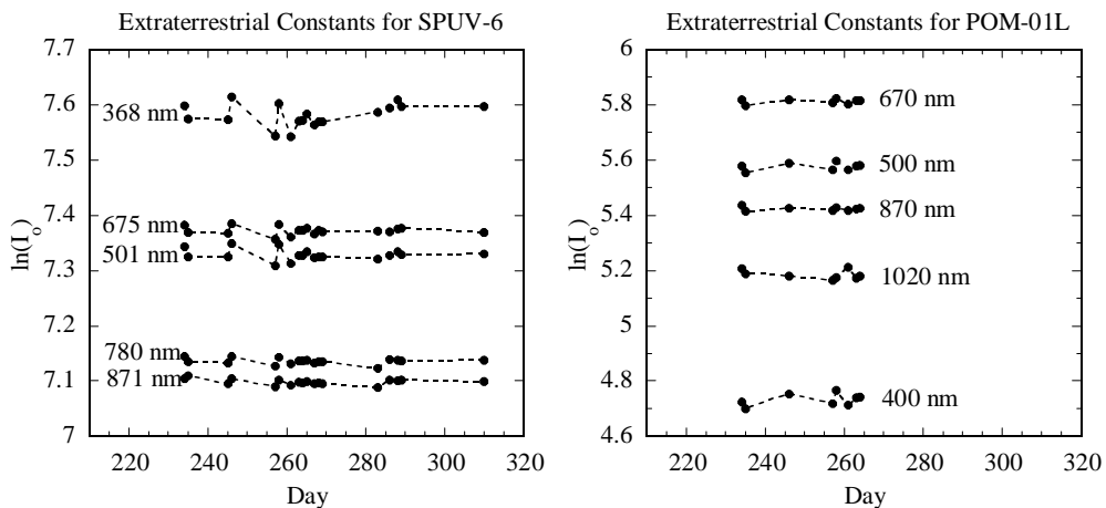
Figure 3: Extraterrestrial Constants for the aerosol channels of the SPUV-6 (left panel) and POM-01L (right panel) for the measurement period. For both data sets the first point corresponds to 22 August 2003. For the SPUV-6 the last point was taken on 6 November 2003, for the POM-01L this was 21 September 2003. The standard deviation of the mean varies between <0.1% and 0.5 %, depending on the channel and the instrument.
